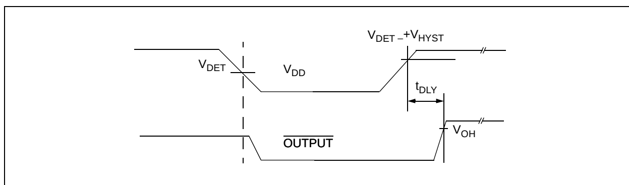
FIGURE 1-1: Timing Diagram.
